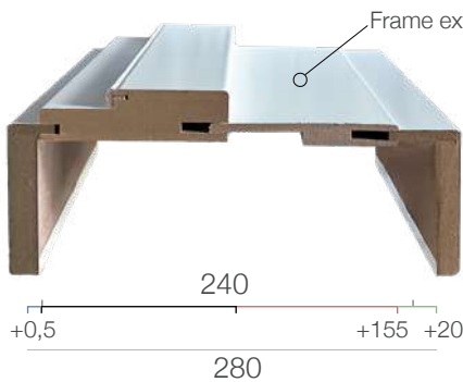
WING 10 + C.BATEX* 100 + FRAME EXTENSION 160 + WING 25
