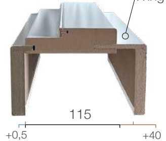
WING 10 + C.BATEX* 100 + WING 45
