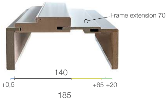
WING 10 + C.BATEX* 100 + FRAME EXTENSION 70 + WING 25
