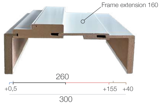
WING 10 + C.BATEX* 100 + FRAME EXTENSION 160 + WING 45
