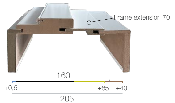
WING 10 + C.BATEX* 100 + FRAME EXTENSION 70 + WING 45
