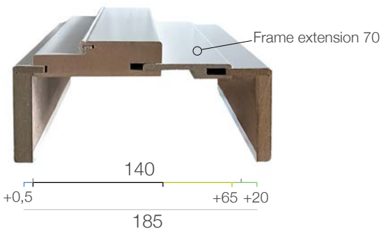
WING 10 + C.BATEX* 100 + FRAME EXTENSION 70 + WING 25
