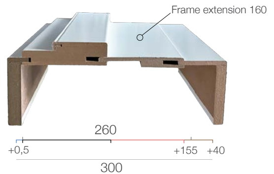
WING 10 + C.BATEX* 100 + FRAME EXTENSION 160 + WING 45
