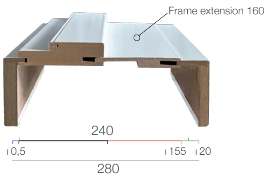
WING 10 + C.BATEX* 100 + FRAME EXTENSION 160 + WING 25
