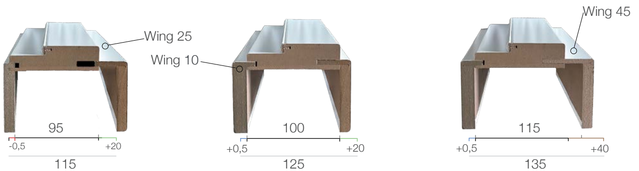
TADAP** + C.BATEX* 100 + WING 25
